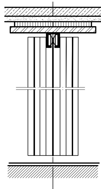
TOP HUNG EXPOSED TRACK
